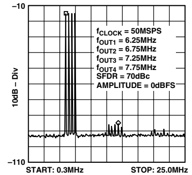
Figure 20. Four-Tone SFDR
